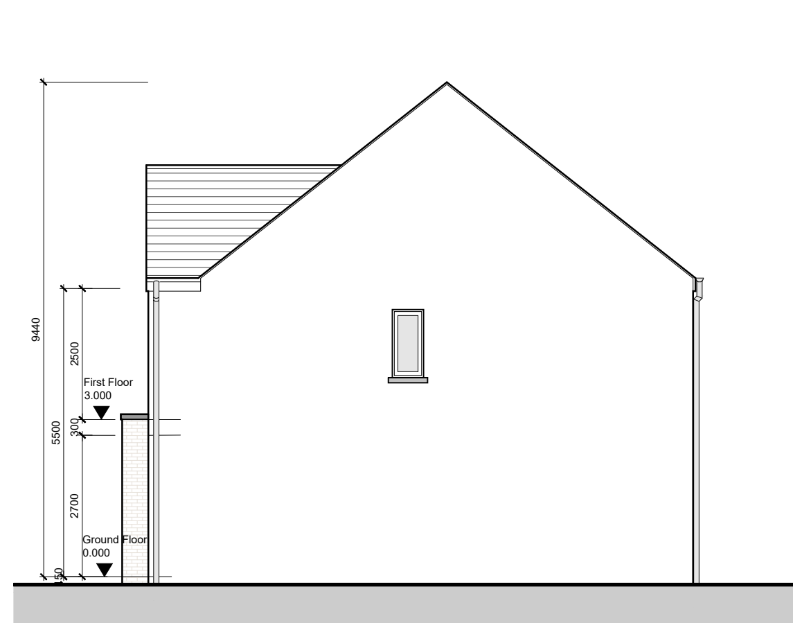
Side Elevation 02
