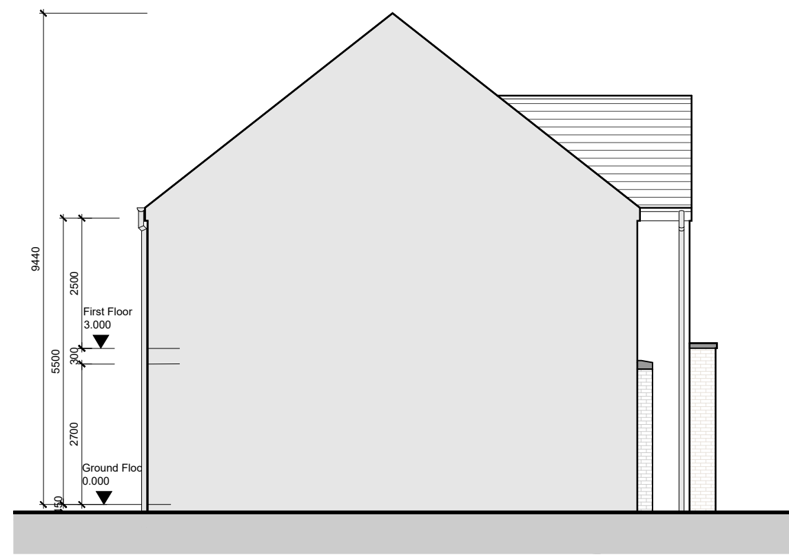
Side Elevation 01
